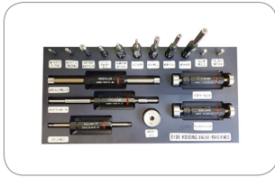
Plug Gauge
